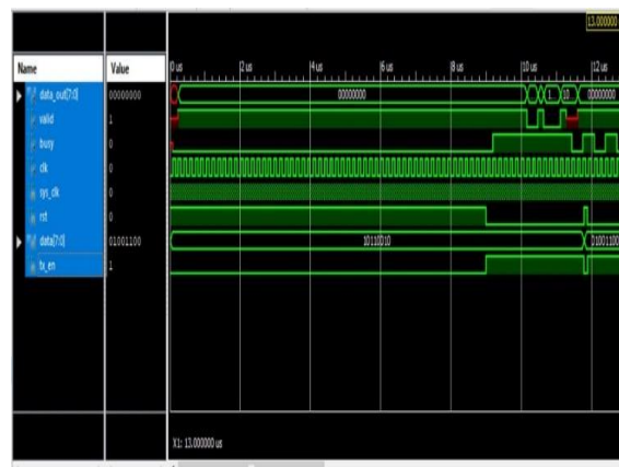
Figure7: UART Output waveform 2
