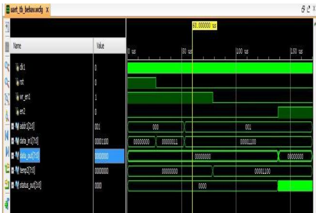
Figure6: UART Output Waveform 1
