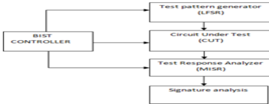
Figure 2: UART with BIST
