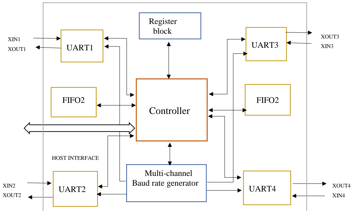
Figure 1: Multi-channel UART
