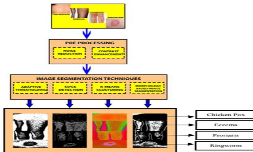
Fig. 1: Work flow diagram of the proposed work
