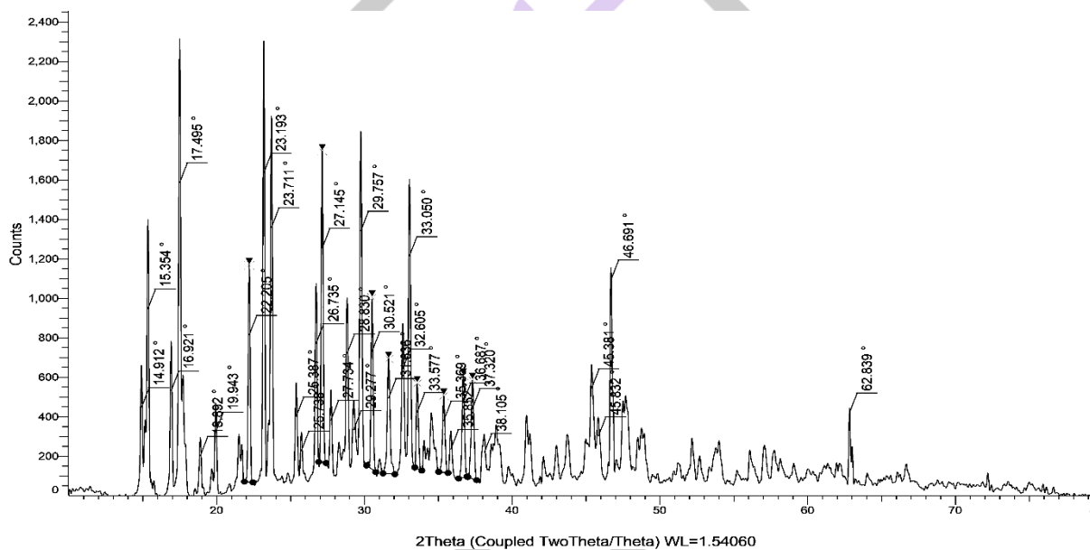
Figure 4: Mirabilis jalapa flower extract iron nanoparticles - X-Ray Diffractogram Fe (Coupled Two Theta/Theta)
