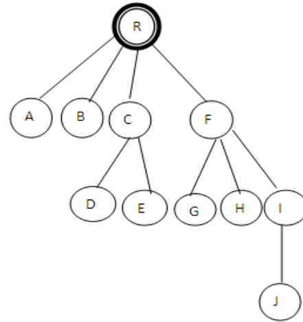
Fig 4.b breadth first spanning tree for node r
