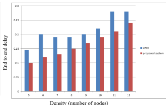
Fig 6.b End to end delay with density
