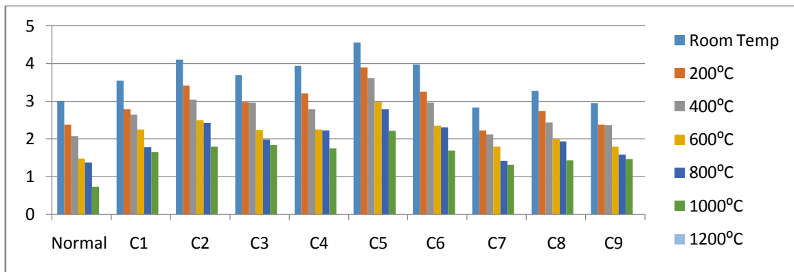
Figure 2. Split Tensile Strength in N/mm 2 (28 days)
