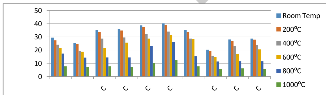
Figure 1. Compressive Strength in N/mm 2 (28 days)
