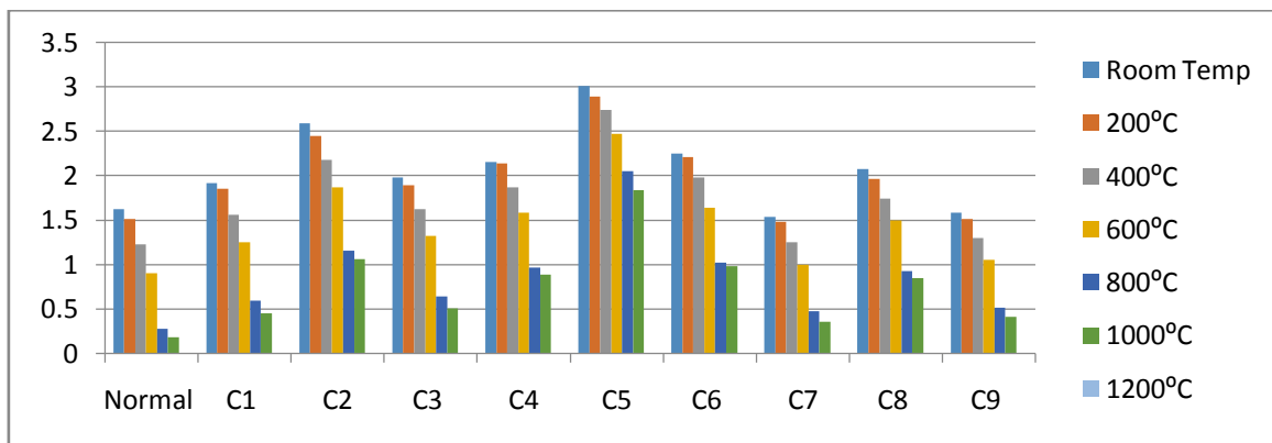
Figure 3. Flexural Strength in N/mm 2 (28 days)
