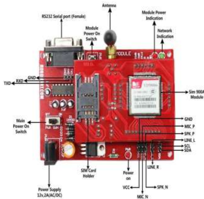
Fig3: GSM sim900A
