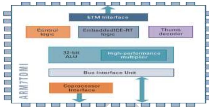
“Figure 1” ARM7TDMI Processor Architecture
