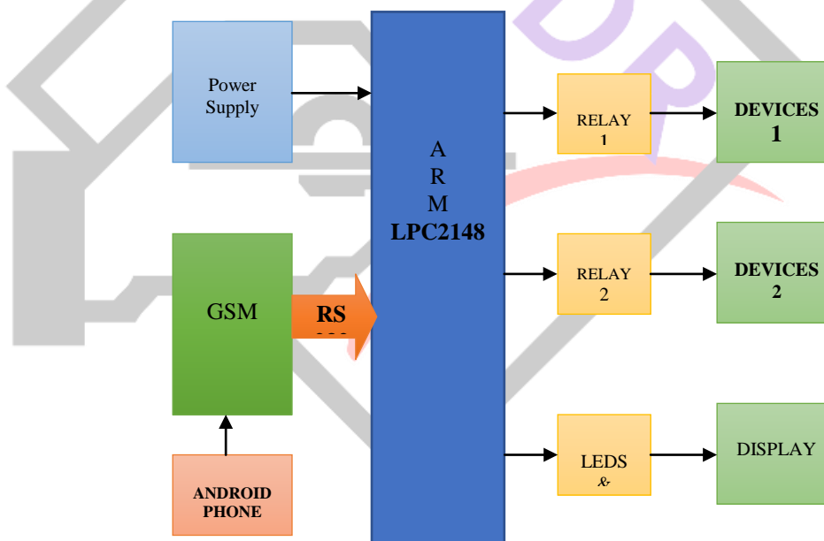
“Figure 4” TOTAL SYSTEM BLOCK DIAGRAM
