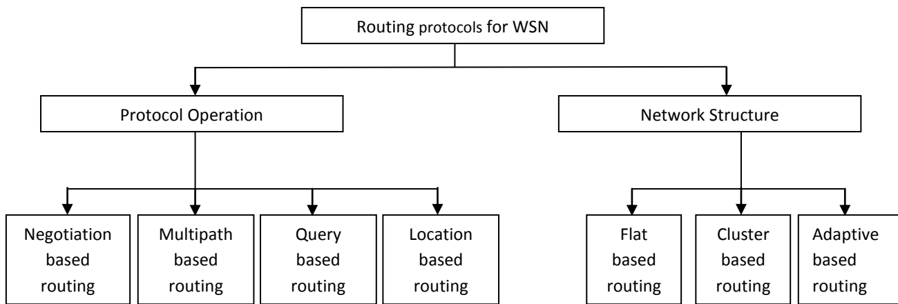
Figure. 1 Taxonomy of routing protocol for WSN
