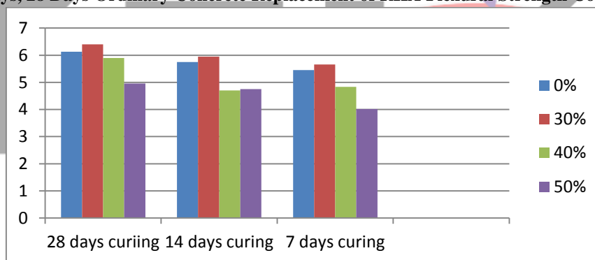
Figure 6.7 7days,14 Days, 28 Days Ordinary Concrete Replacement of RHA Flexural Strength Comparison Results
