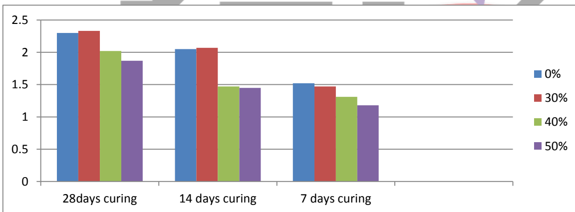
Figure 6.5 7days, 14 Days, 28 Days Ordinary Concrete Replacement of RHA Split Tensile Strength Comparision Results
