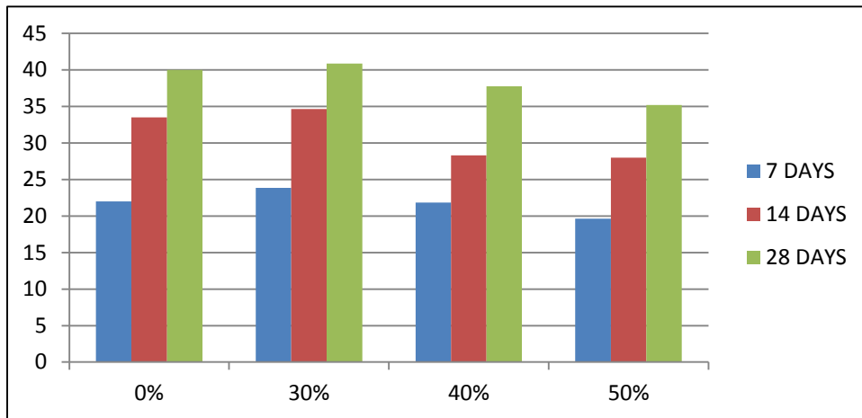
Figure 6.3 Compressive Strength Result Comparision of Ordinary Concrete & Self Compacting Concrete
