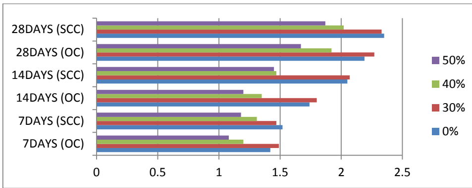
Figure 6.6 Split Tensile Strength Result Comparison of Ordinary Concrete & Self Compacting Concrete
