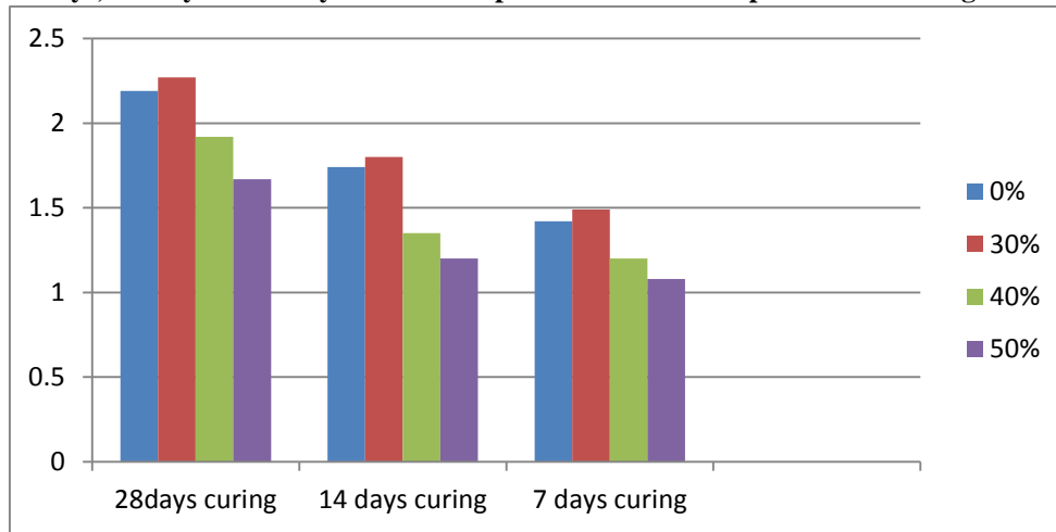
Figure 6.4 7days, 14 Days, 28 Days Ordinary Concrete Replacement of RHA Split Tensile Strength Comparision Results
