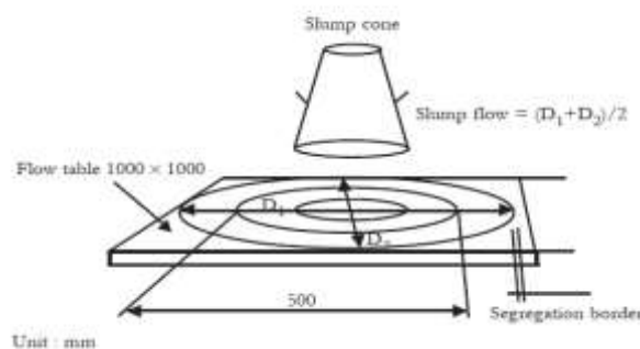
Fig.5.1 Slump Flow Test
