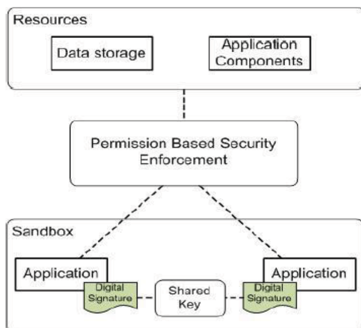
Fig 2: Android Security Model [10]
