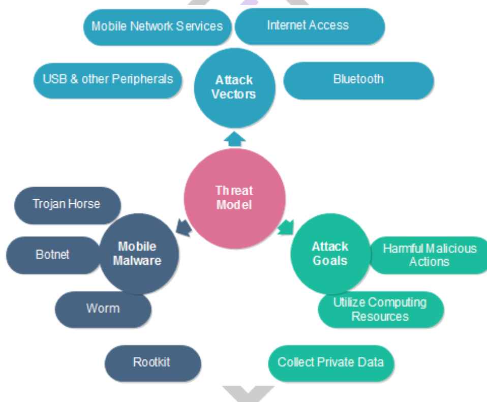
Fig 1: Mobile Platform Model Threats (MPMT) [10]
