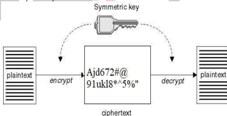
Fig 2: Symmetric Encryption
