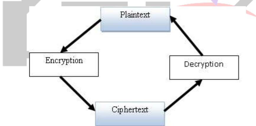
Fig 1: Cryptography Process
