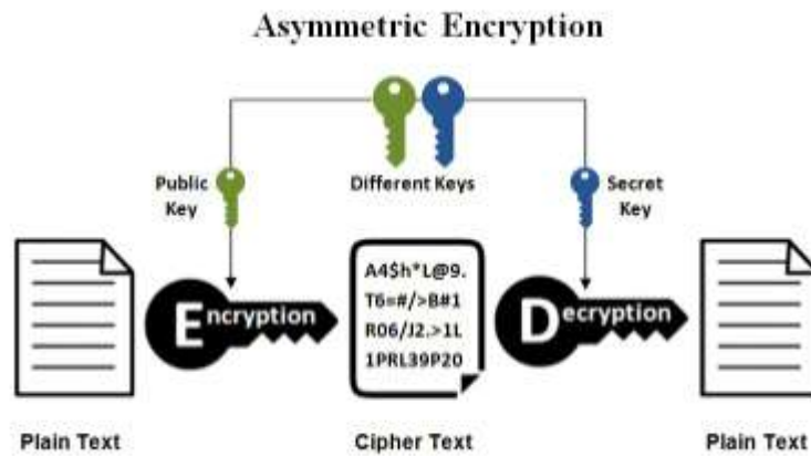
Fig 3: Asymmetric Encryption
