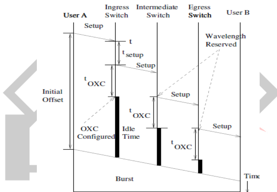
Figure 3 : Just-In-Time Reservation Scheme
