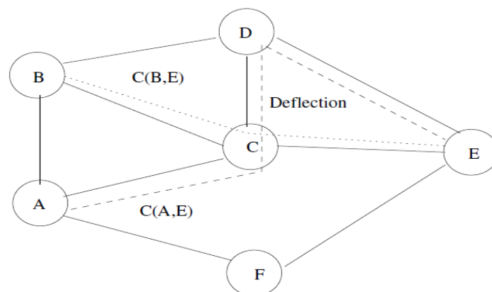
Figure 7 : Deflection routing.
