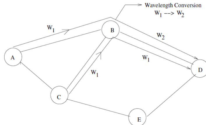
Figure 6 : Wavelength conversion
