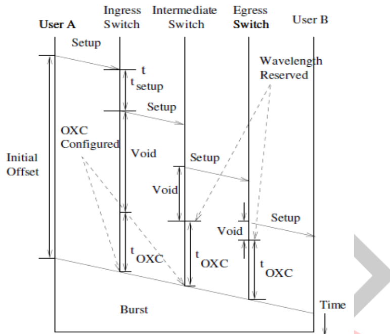
Figure 4 : Just-Enough-Time Reservation Scheme
