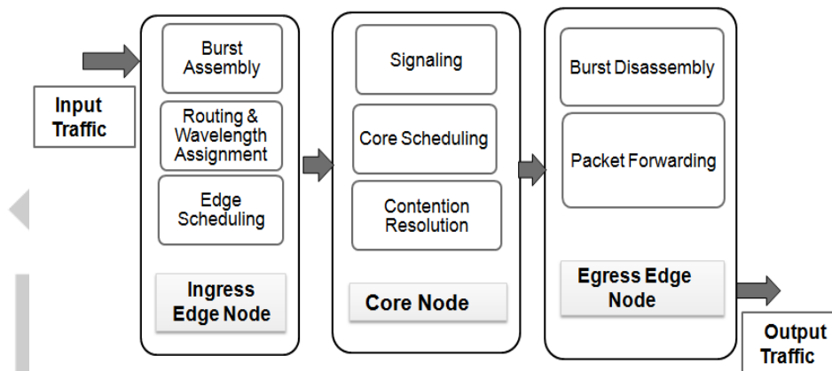
Figure 1: OBS Functional Diagram
